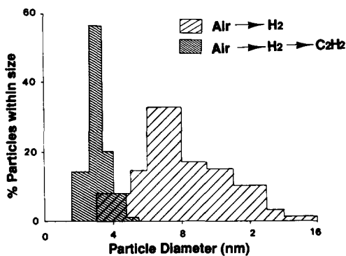
FIG. 7. Particle size distribution of a model platinum/alumina catalyst after heating to 500°C in (a) air for 2.0 h, (b) hydrogen for 4.0 h, and (c) acetylene for 0.5 h.
